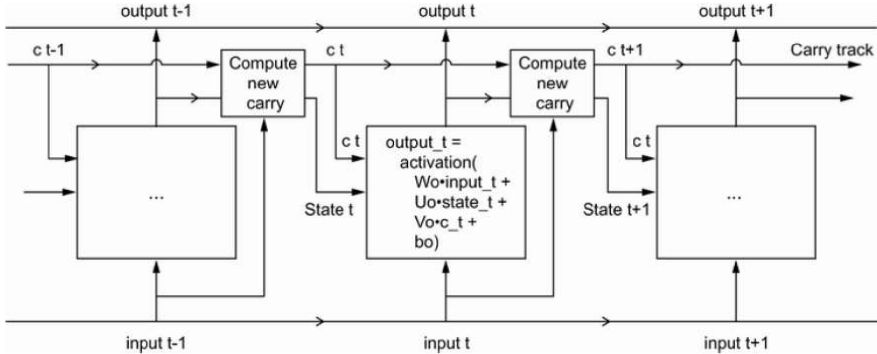
Figure 10.10 Anatomy of an LSTM
